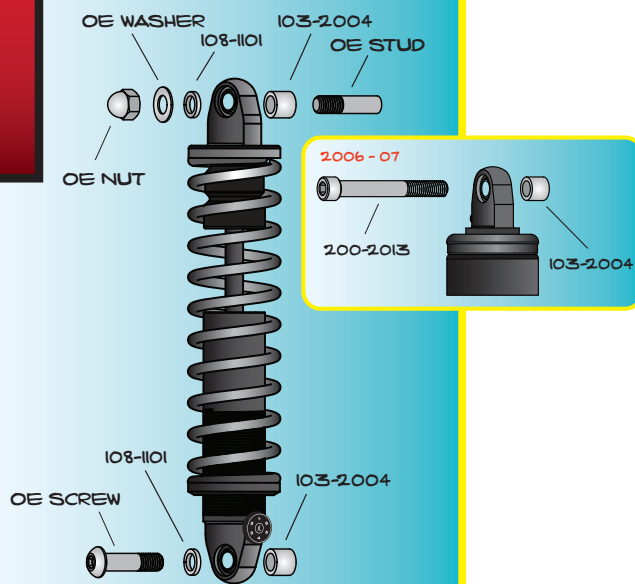
FIGURE A - 2008+ (LEFT SHOCK)
